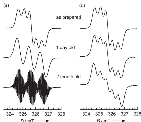
Figure 1. Temporal ESR spectral changes of 1^+ in a) \text{CH}_2\text{Cl}_2 (recorded at 295 K) and b) n -butyronitrile (recorded at 293 K).
